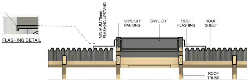
METAL ROOF SECTION 2 SCALE: 1 : 20
