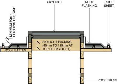
FLAT ROOF SECTION 2 SCALE: 1 : 20
