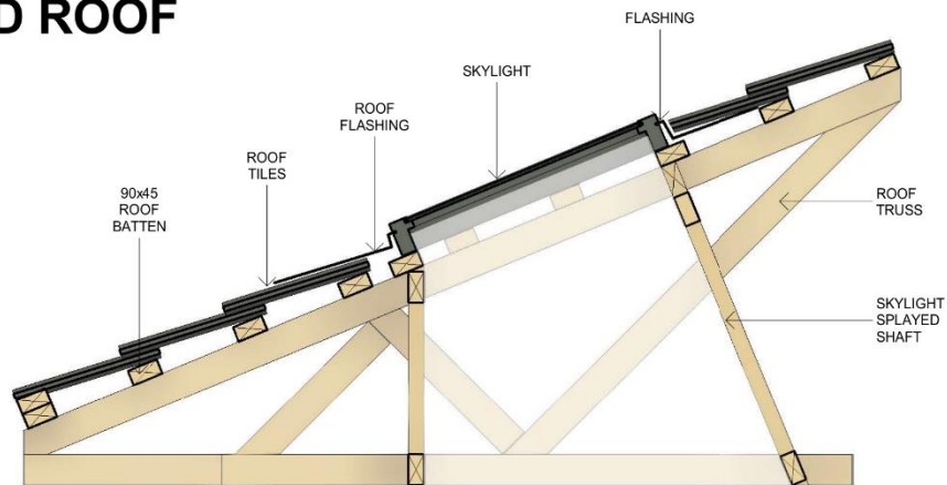
TILED ROOF SECTION 1 SCALE: 1 : 20
