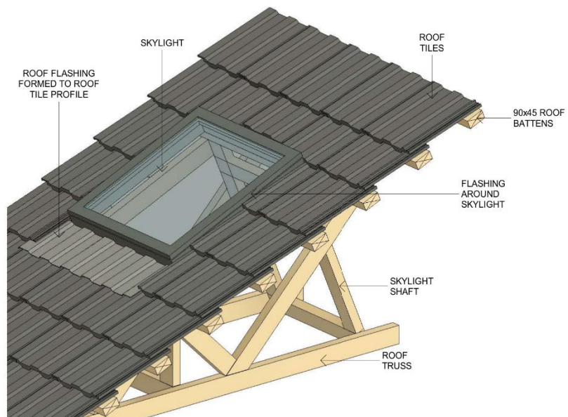
TILED ROOF SECTION 2 SCALE: 1 : 20
